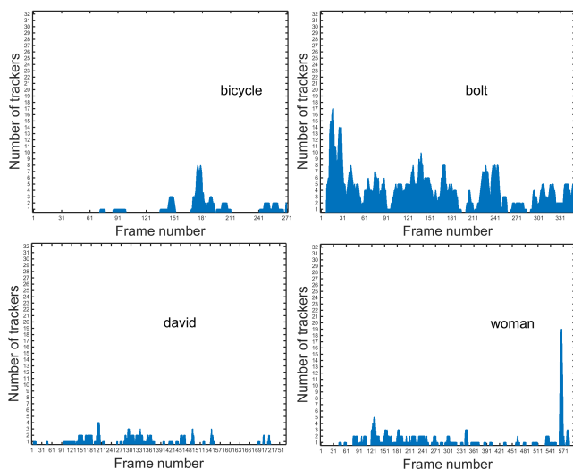
Fig. 11. Difficulty curves for the bicycle , bolt , david , and woman sequences.
