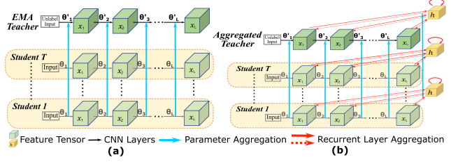
Figure 5. The illustration of (a) EMA Teacher and (b) our Aggregated Teacher. EMA teacher performs aggregation only over parameters, while our Aggregated teacher performs aggregation over both parameters and layers.
